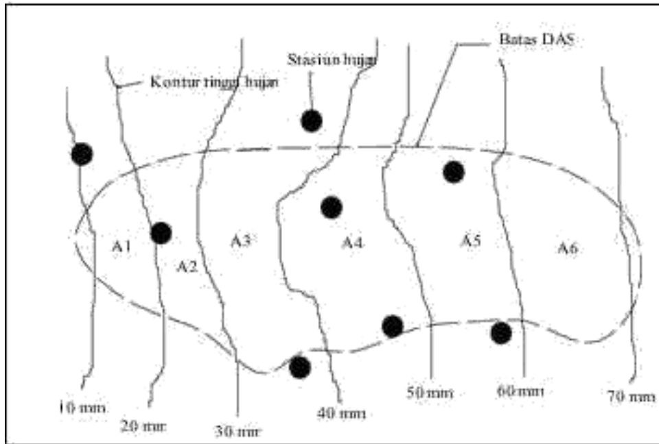
Gambar 2.5. Metode Isohyet (Soemarto, 1999)
