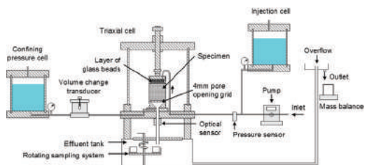
Figure 1. Schematic diagram of the triaxial erodimeter.
