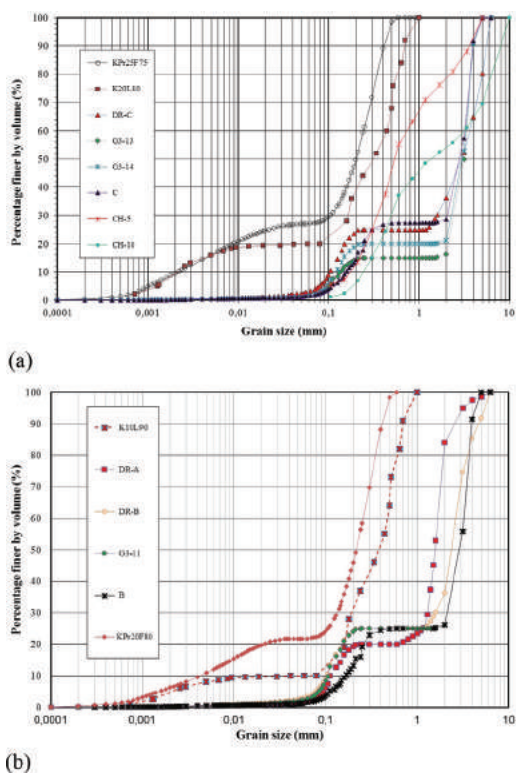
Figure 2. Grain size distribution of tested soils, (a) soils KPr25F75, K20L80, DR-C, G3-13, G3-14, C, CH-5, CH-10, (b) soils K10L90, DR-A, DR-B, G3-11, B, KPr20F80.
