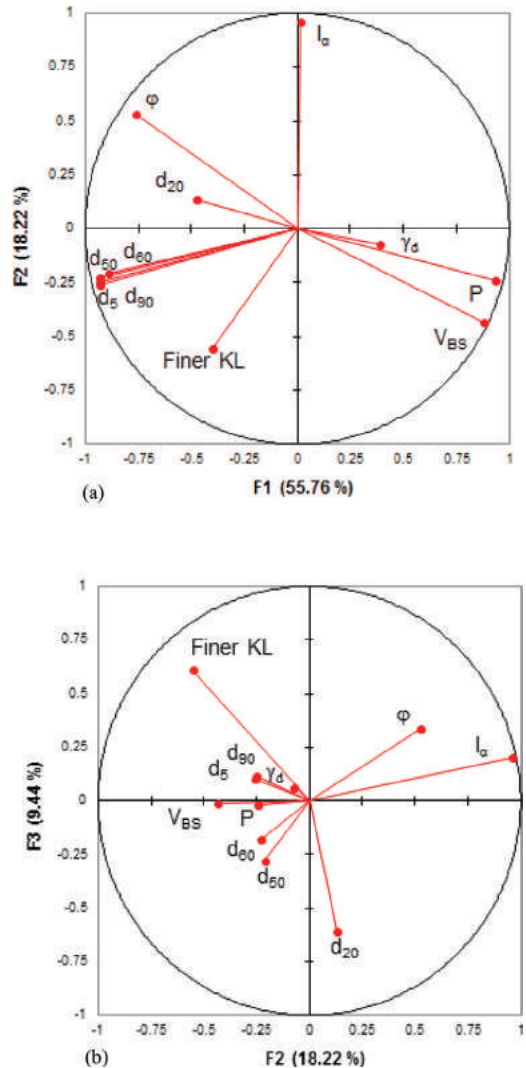
Figure 4. Representation of variables in: (a) factor plane 1-2, (b) factor plane 2-3.
