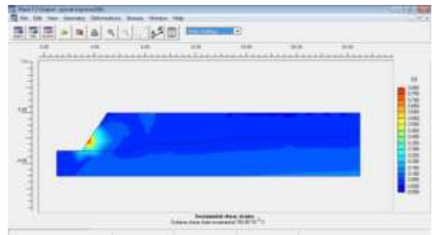
Figure 11 Sliding pattern 1
