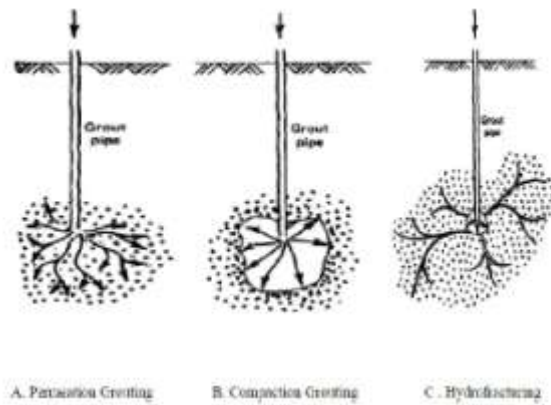
Figure 5 Types of grouting system 6
