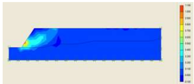
Figure 9 Incremental strains after heavy rain 1
