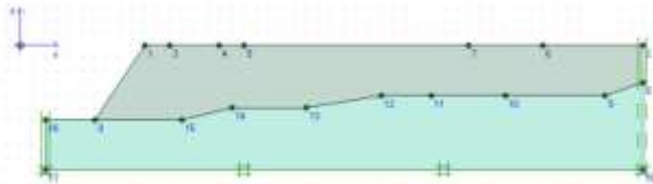
Figure 6 Plaxis 7.2 model for fill and slope 1
