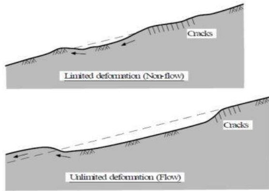
Figure 4 Flow and non-flow deformation of sandy soil 2
