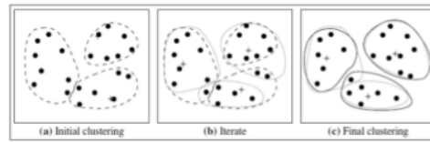
Gambar 2. 1 K-Means Clustering [10]
