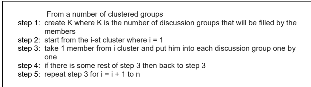
Figure 1. Modeling in Pseudo-code Form
